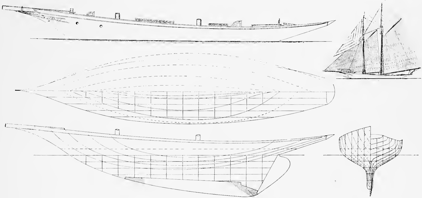
COMPOSITE SCHOONER YACHT.—Designed by Fred. W. Martin, Superintendent of the Racine (Wis.) Yacht and Boat Works.
